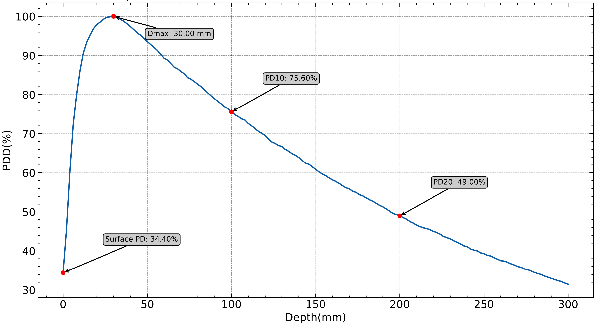
PDD profile of 6MV FFF SSD=100, Water Phantom, F.S= 10x10cm 2
